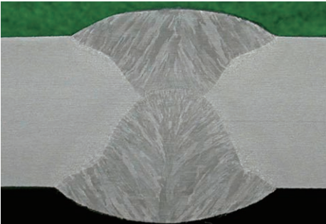
Photo. Macro structure of I-Butt joint (T=13mm)
