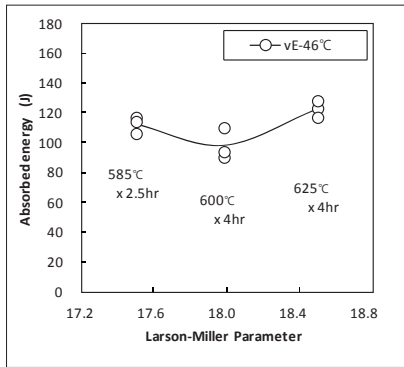
Fig. Charpy impact properties of deposited metal (PWHT, vE-46℃)
